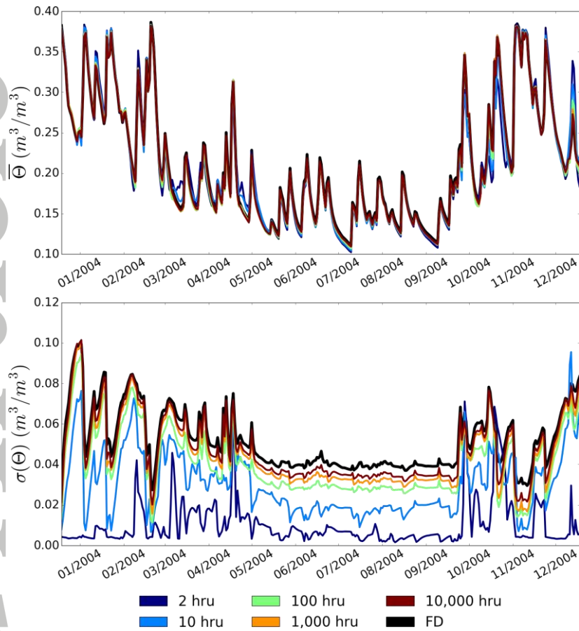
Figure 6. Modeled catchment soil moisture mean and standard deviation using HydroBlocks with 2, 10, 100, 1,000, and 10,000 HRUs and the fully distributed model over the Little Washita watershed.
